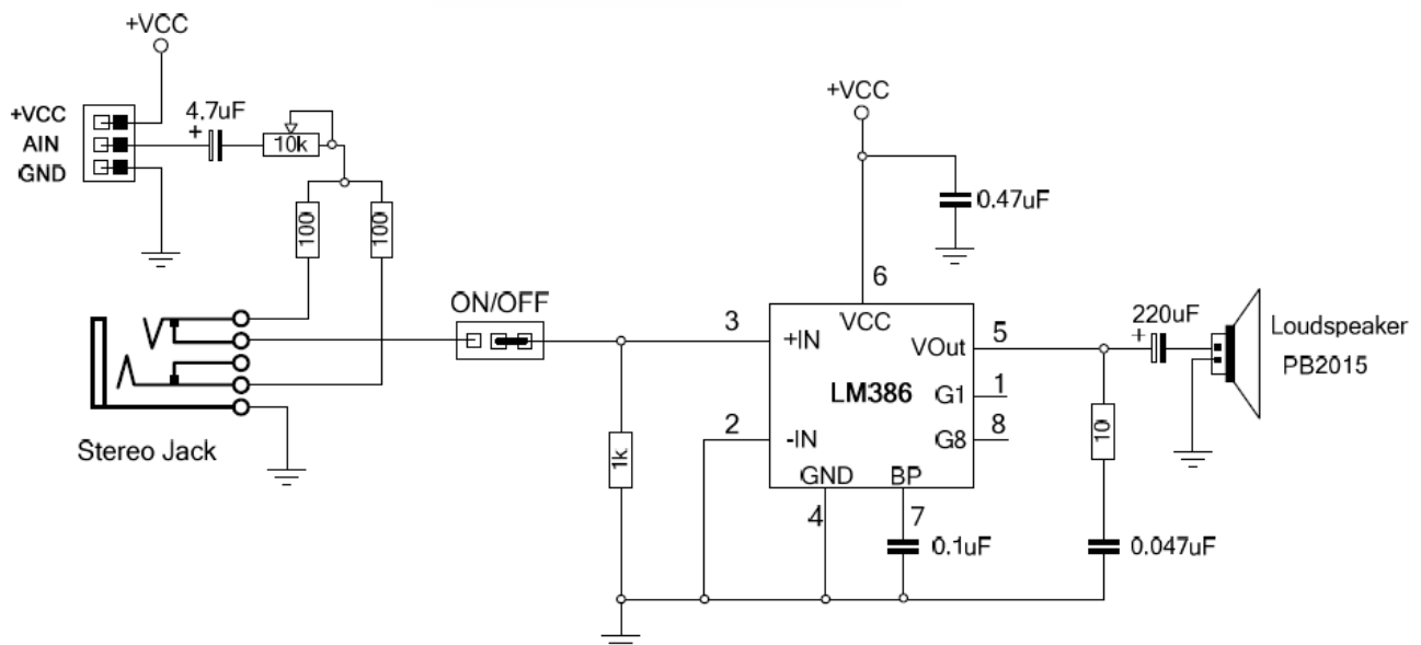
FIG 2: MR-MINI-AUDIO Schematic
