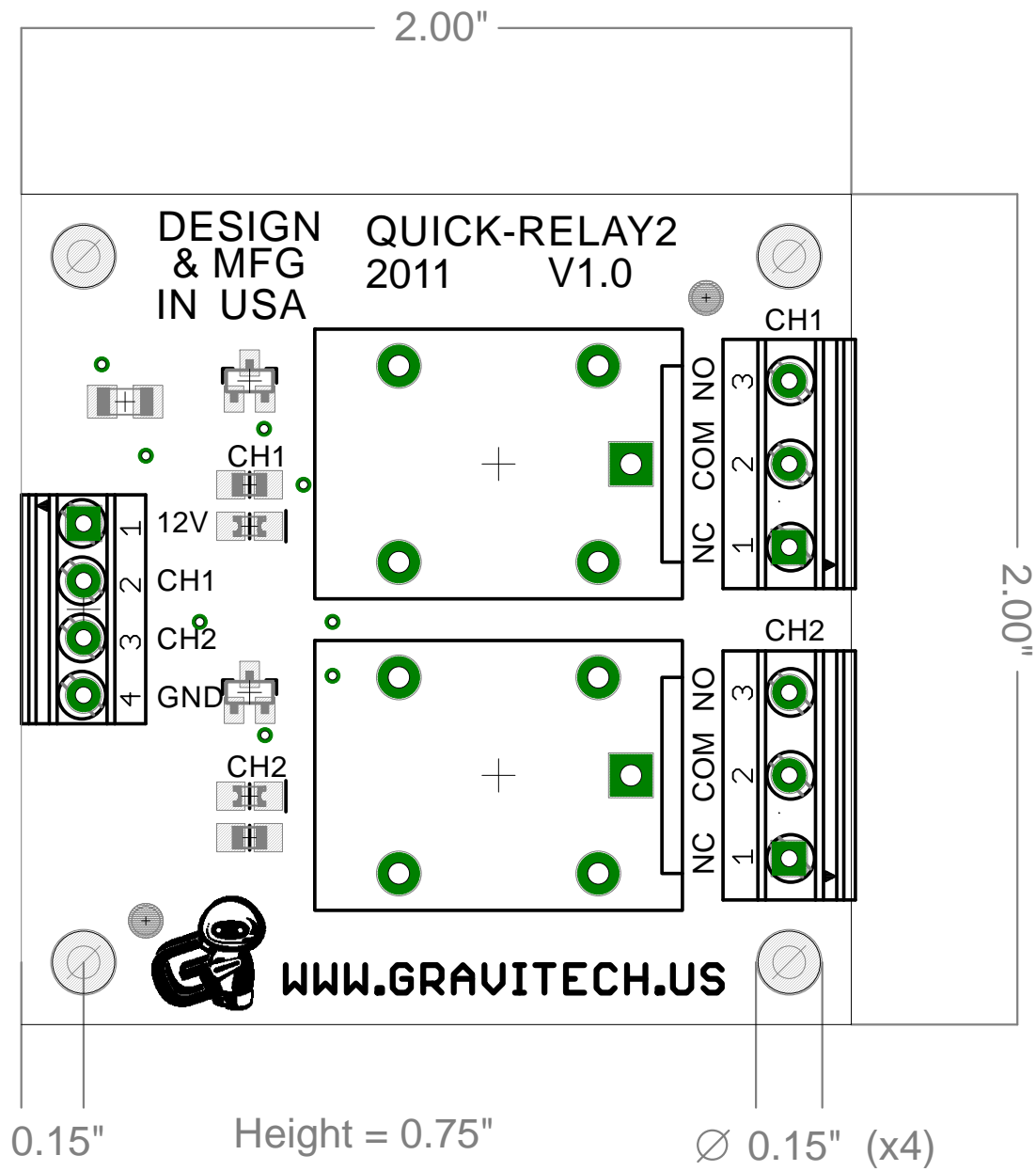
QUICK-RELAY2 MECHANICAL DIMENSIONS
